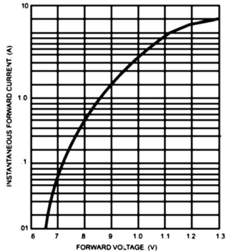
FIG.3- TYPICAL FORWARD VOLTAGE
